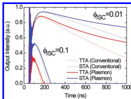
Figure 4. Output intensity from an OSL, using the parameters given in Table 1, excited with a square pulse of t_R = 35 ns rise time, at an excitation rate R = 1.5R_{\text{th}0} . The transient emission is shown for the case of triplet–triplet absorption (TTA) and singlet–triplet annihilation (STA). In both cases, the laser emission is short-lived. Also shown is the transient emission for a reduced triplet lifetime due to the presence of the plasmonic sink. It is found that the reduced triplet lifetime does not significantly affect the short time dynamics.
